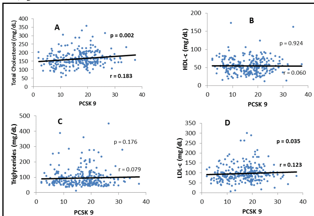
Figure 1. Correlation between PCSK9 and lipid profile in the study population A: Correlation between PCSK9 and total cholesterol; B: Correlation between PCSK9 and HDL-c; C: Correlation between PCSK9 and triglycerides; D: Correlation between PCSK9 and LDL-c
